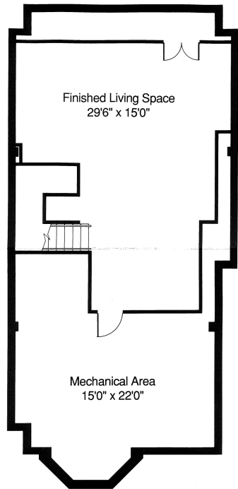
BASEMENT 600 sq. ft.
