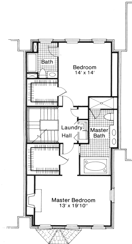
SECOND FLOOR 1,200 sq. ft.
